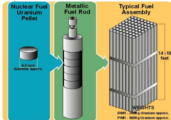
Figure B. Typical Fuel Assembly
