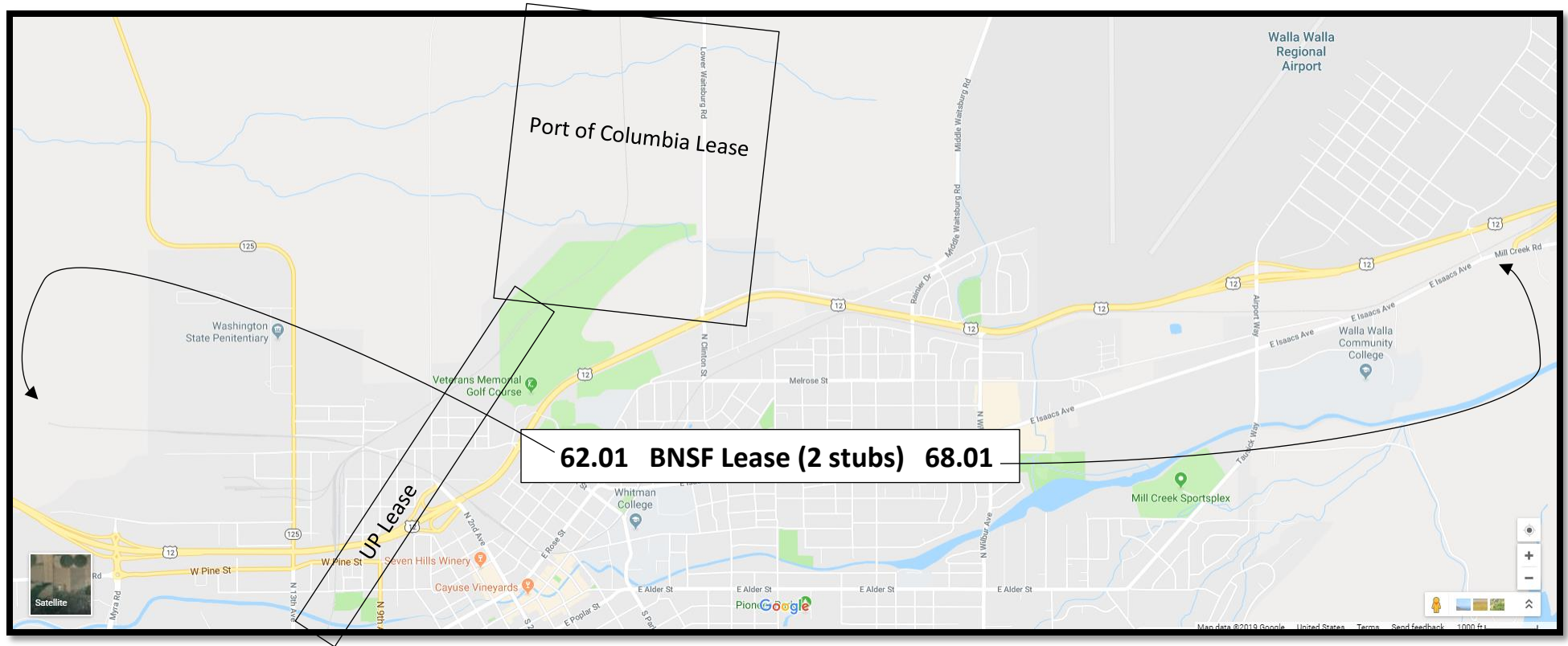
FD 36304 EXHIBIT A-1 Map of CWW Leasehold in Walla Walla, WA (BNSF-owned track):
