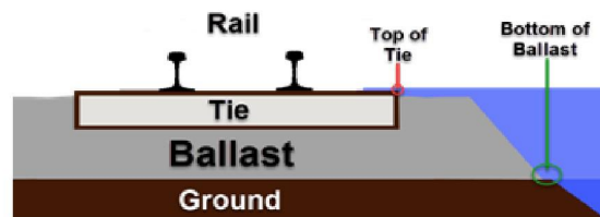
Figure 1 - Top of Tie and Bottom of Ballast
